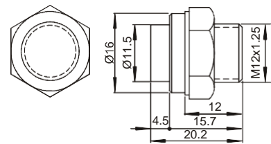
Sizes of the M12x1.25 stapled fitting
